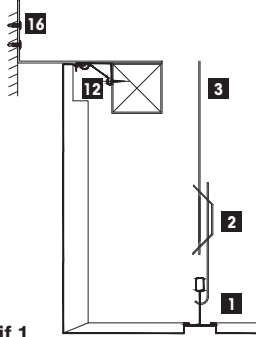
1-1 Kesiti / Section 1-1
