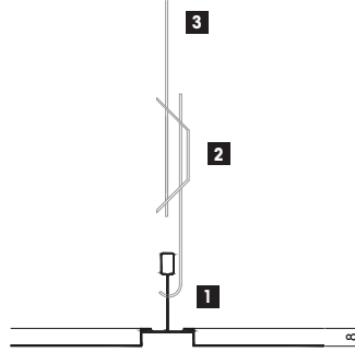
1-1 Kesiti / Section 1-1
