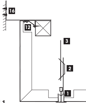
1-1 Kesiti / Section 1-1
