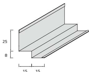
25 X 8 X 15 X 15 W 3002/B - W 3002/N - W 3002/M steel 0.5 mm
