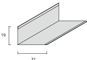
31 X 19 CP60 aluminum 0.5/0.6 mm A 3003/B - A 3003/N - A 3003/M steel 0.5 mm
