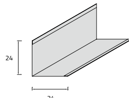
24 X 24 CP 10/1 aluminum 0.5/0.6 mm A 3001/B - A 3001/B.1 - A 3001/N - A 3001/M steel 0.4/0.5 mm
