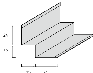
24 X 15 X 15 X 24 W 3004/B - W 3004/N - W 3004/M steel 0.5/0.6 mm
