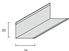
24 X 20 CP 10 aluminum 0.5/0.6 mm A 3000/B - A 3000/B.1 - A 3000/N - A 3000/M steel 0.4/0.5 mm
