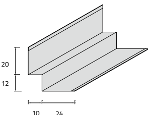
20 X 12 X 10 X 24 CF 10 aluminum 0.5 mm W 3000/B - W 3000/N - W 3000/M steel 0.5 mm
