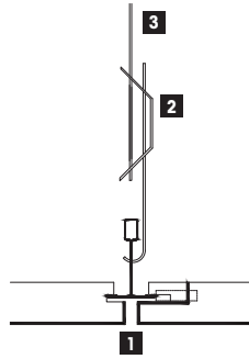
1-1 Kesiti / Section 1-1
